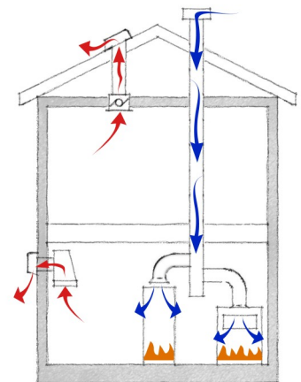
Figure 4. Back Drafting
